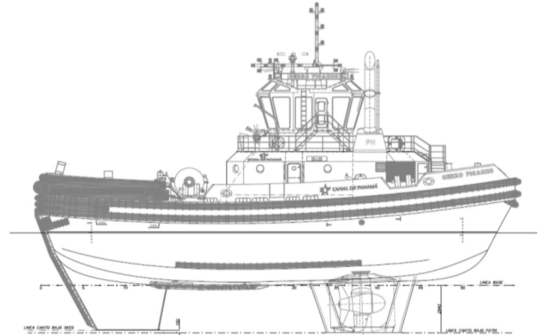
Azimuth Tractor Tug
